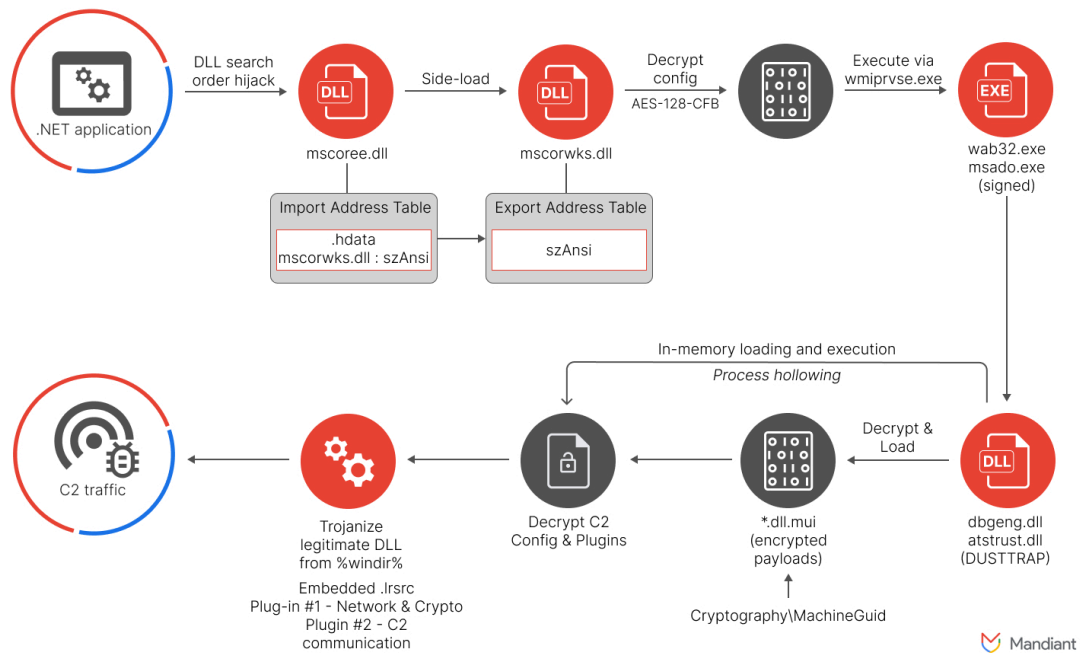
Figure 3: Full execution flow of DUSTTRAP
