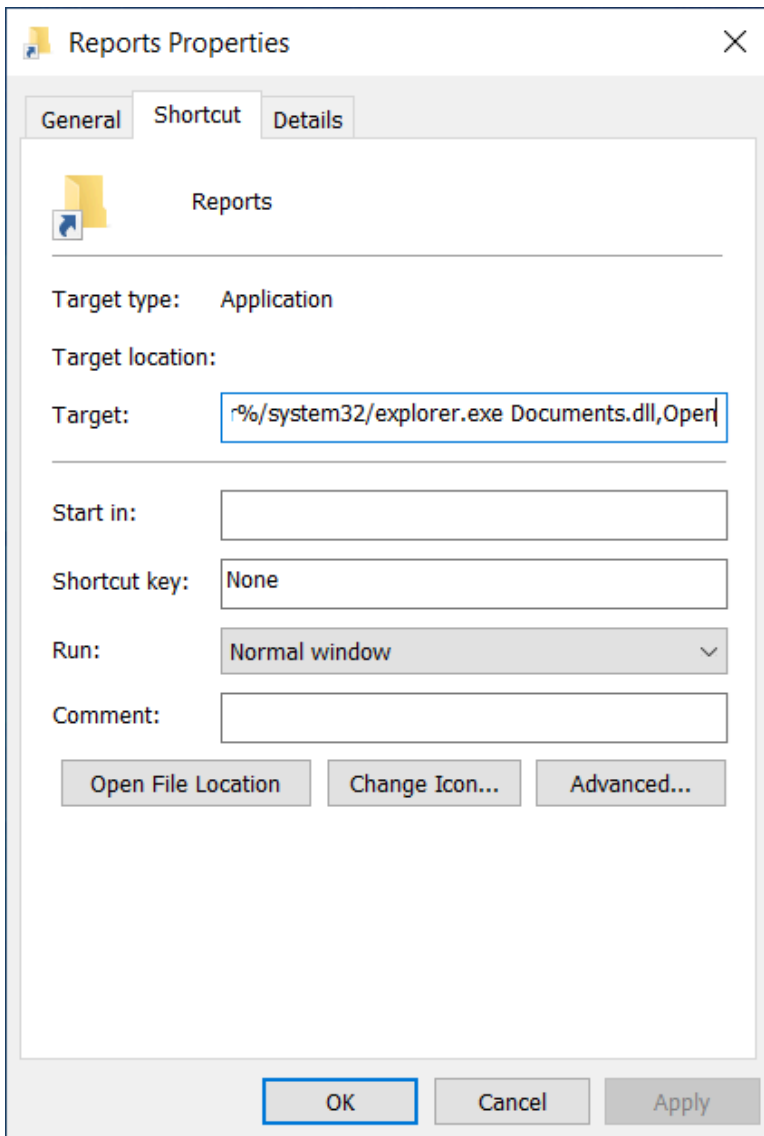
Figure 4. Shortcut which executes the hidden DLL file.
