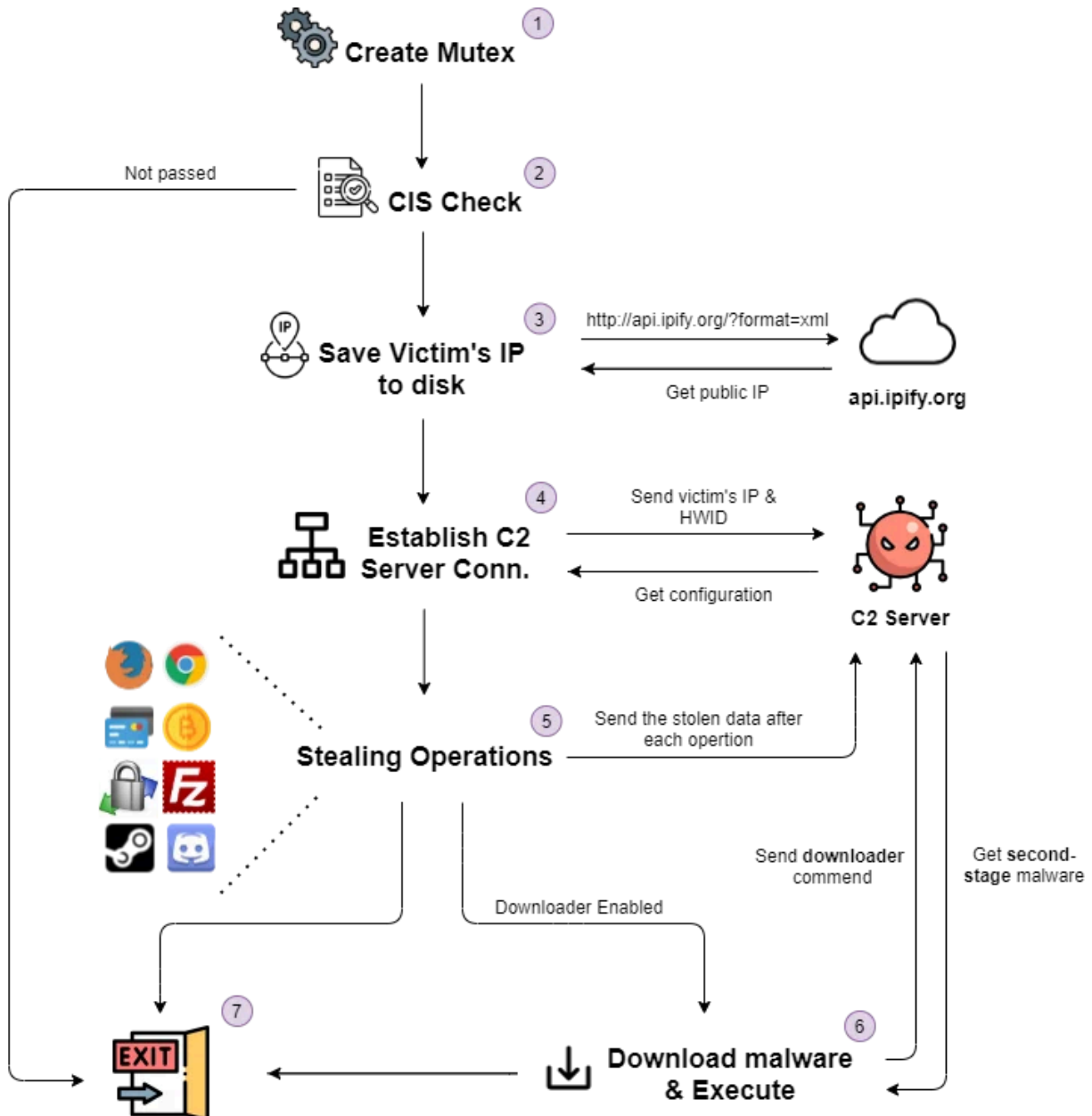
Figure 4: Malware flow
