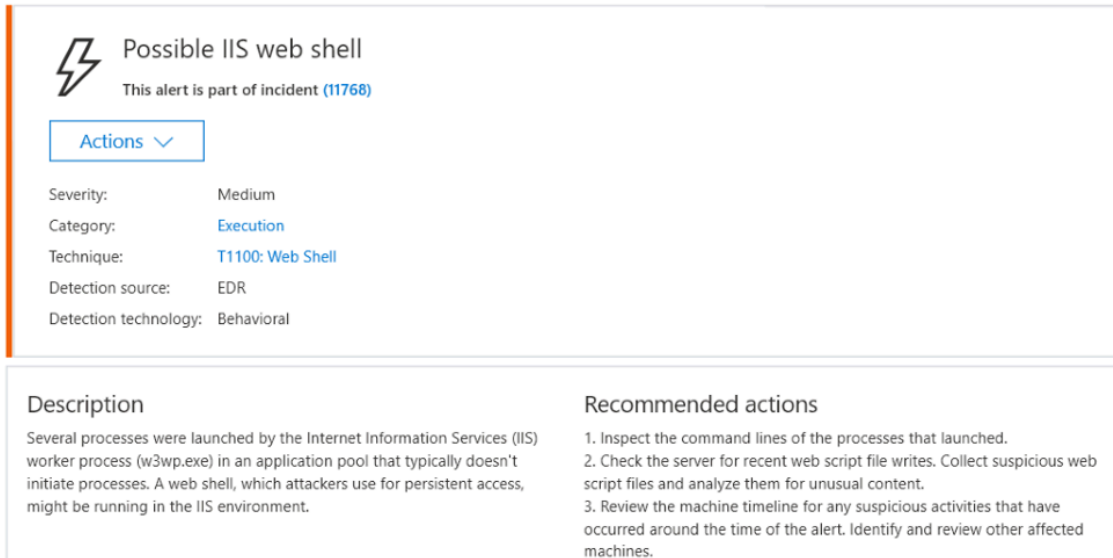
Figure 6: Microsoft Defender for Endpoint alerts of suspicious web shell attacks.
