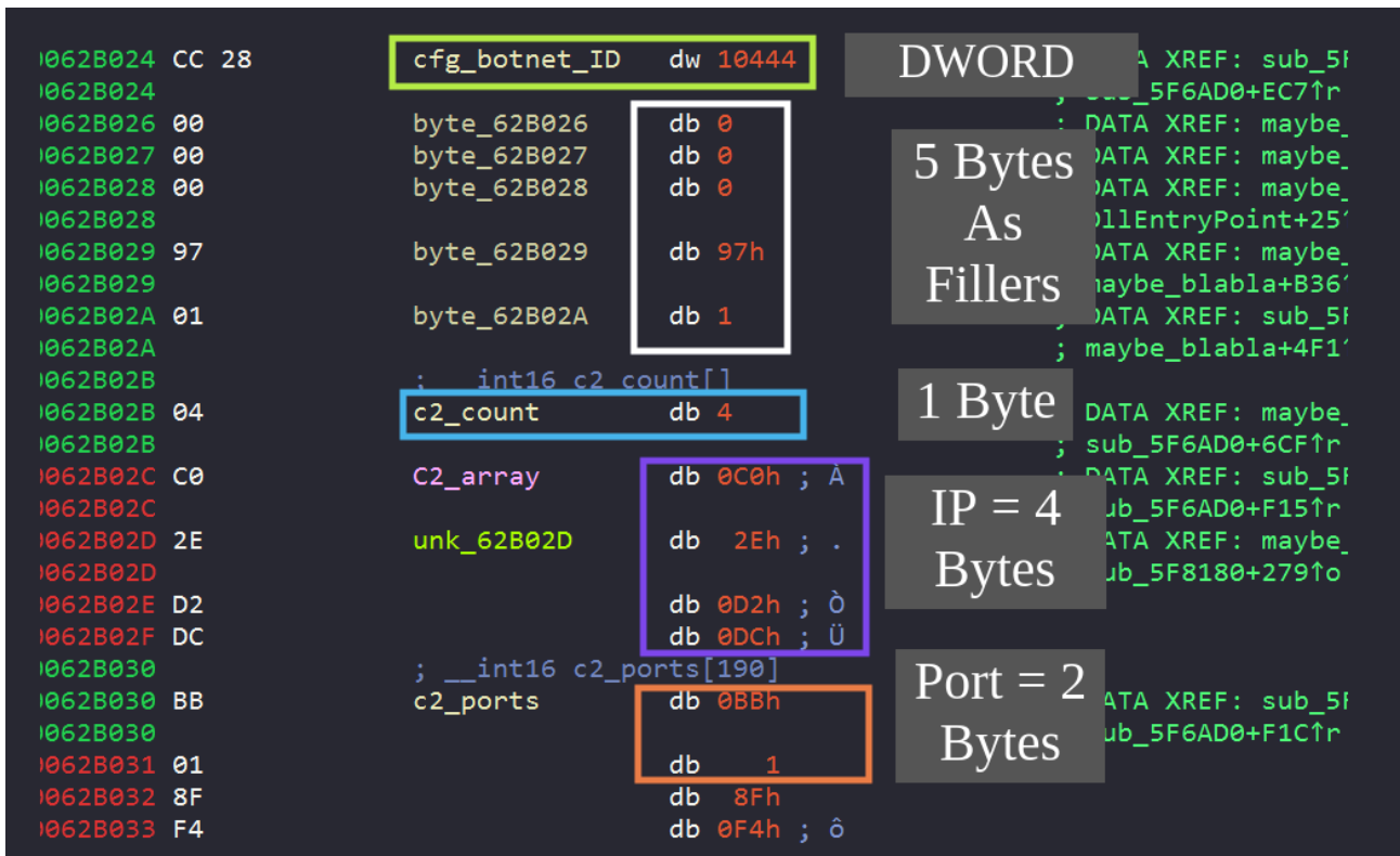
Figure(12): This pattern is repeated starting from (c2_array) to store the whole 4 IPs and their associated ports.
