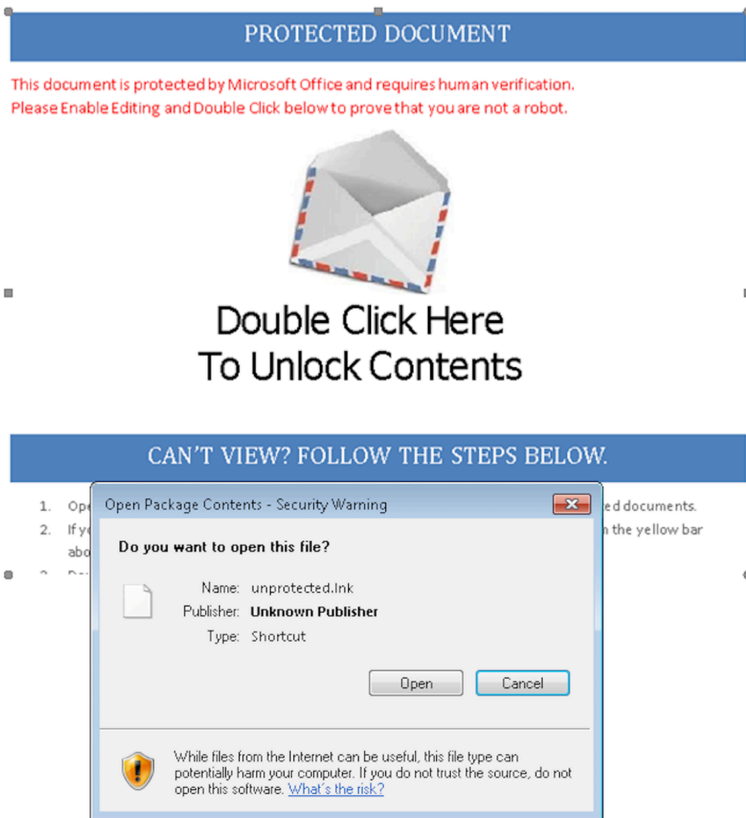
Figure 1: Malicious FIN7 lure asking victim to double click to unlock contents
