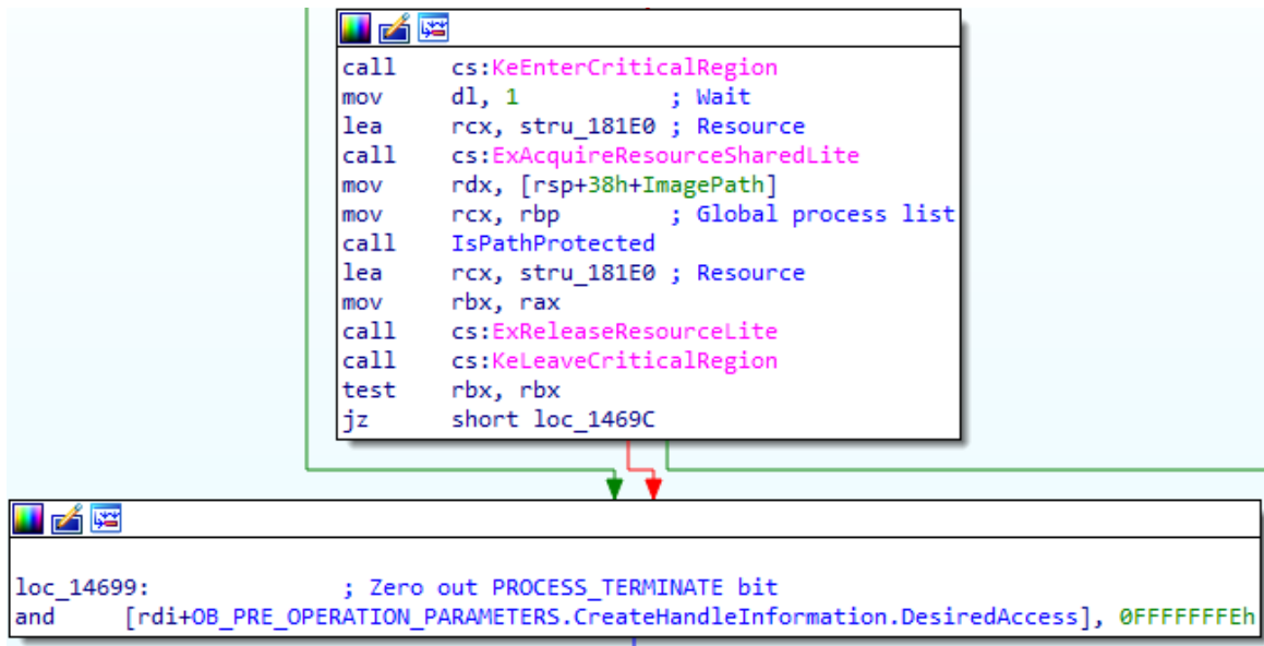
Figure 10: Unsetting the PROCESS_TERMINATE bit of DesiredAccess
