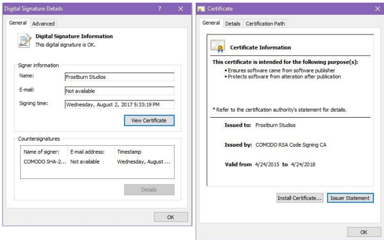
Figure 8: Digital signature of a crtsys.sys driver Two of the samples are on VirusTotal and have a very low detection rate.
