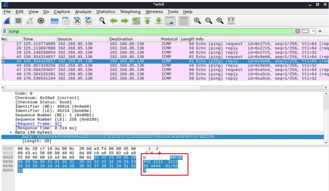
Figure 17 — ICMP data exfiltration packet capture.
