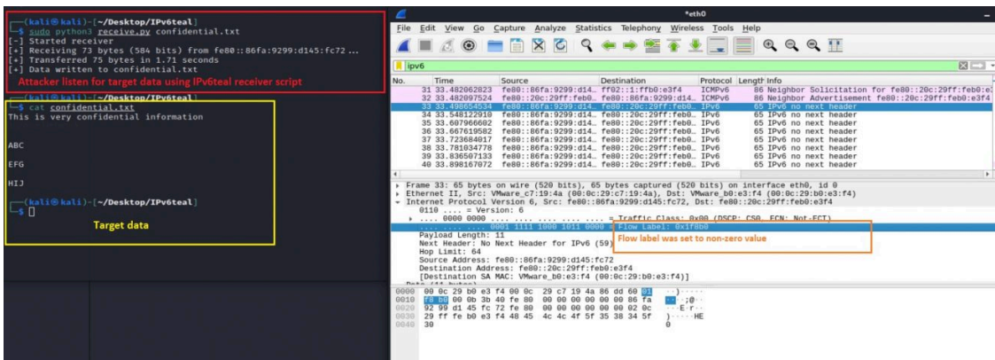
Figure 23 — ‘IPv6teal receiver script’ and related streams.
