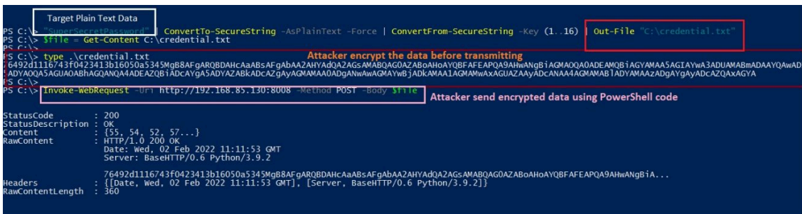
Figure 5 — Victim host to attacker control system communication with encrypted Payload using HTTP POST.
