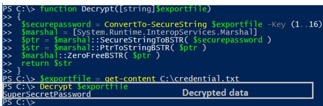
Figure 7 — Encrypted payload/data decryption.
