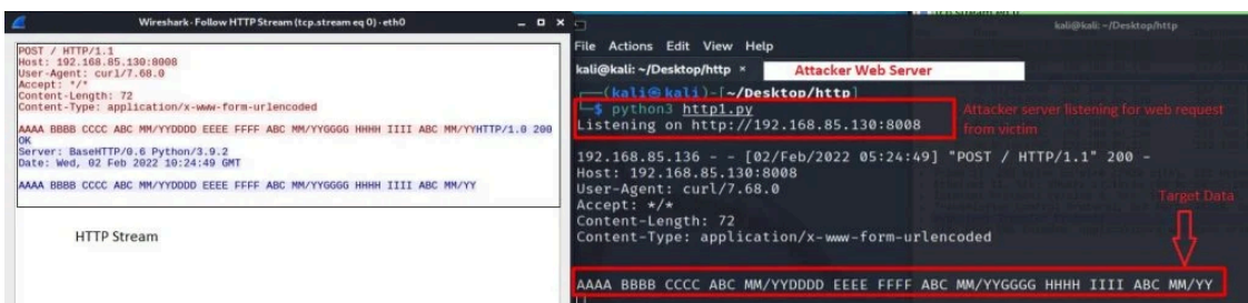
Figure 2 — Attacker server response with cURL POST command executed from the victim host.
