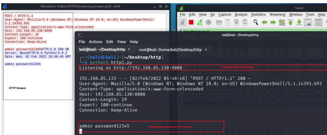
Figure 4 — HTTP POST received from the victim to the attacker listing server.
