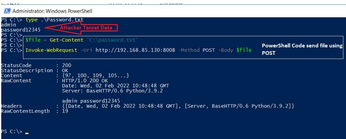
Figure 3 — PowerShell code for HTTP POST from the victim host.
