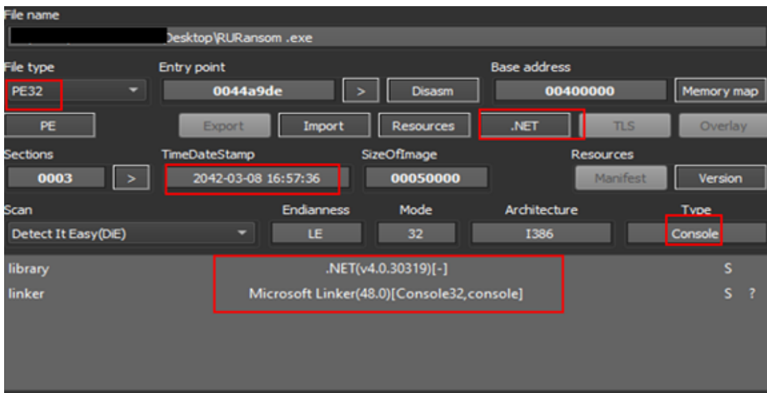
Figure 2: File Info of RURansom Malware
