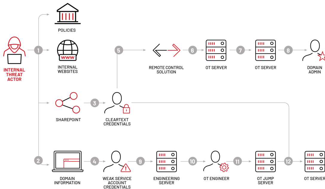
Figure 2: Red Team attack path using FIN11 techniques
