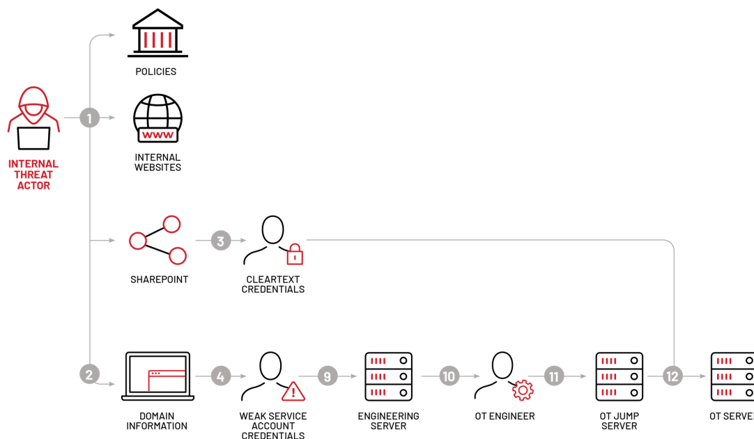
Figure 4: Red Team attack path for OT Compromise #2
