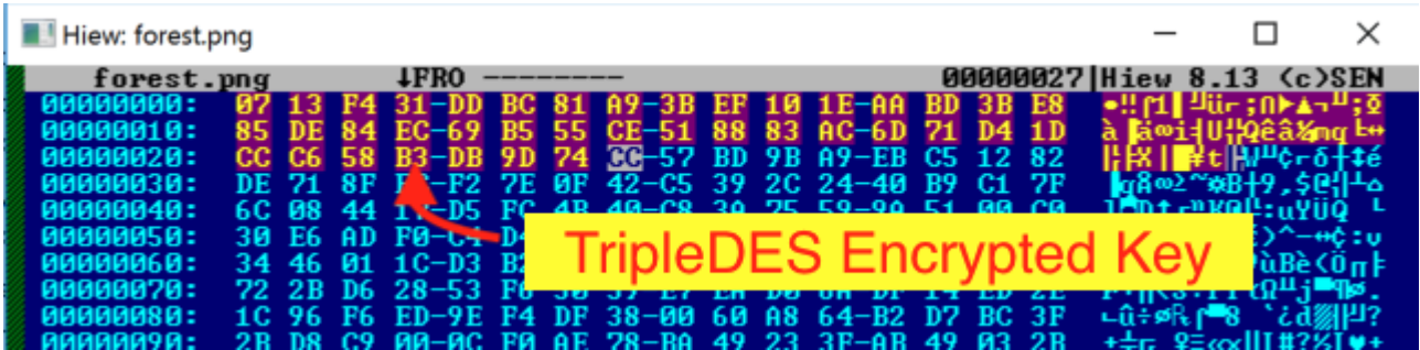
Figure 12: TripleDES encrypted key in the first 40 bytes of the file
