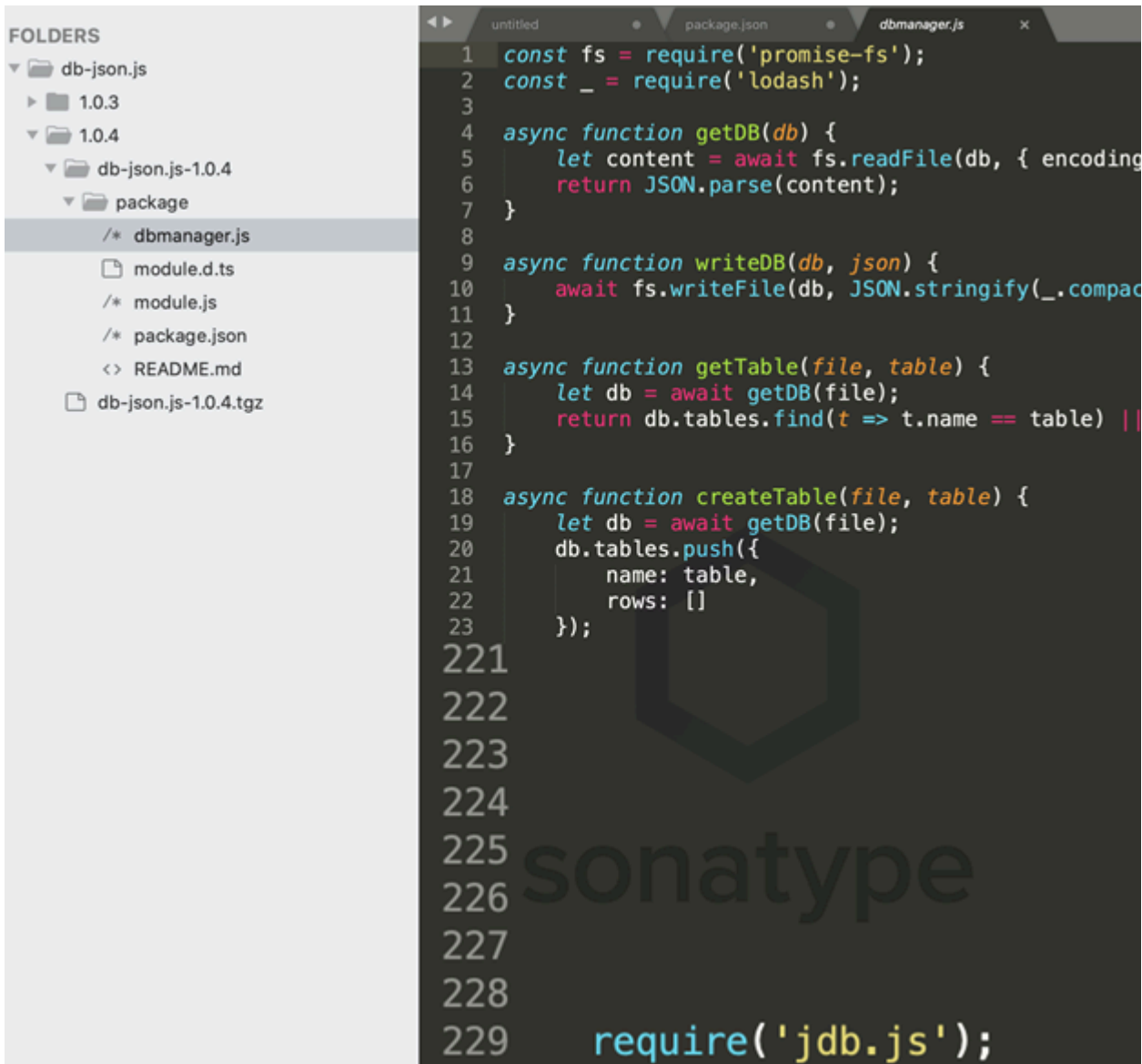
Image: db-json.js containing otherwise "clean" code secretly launches jdb.js
