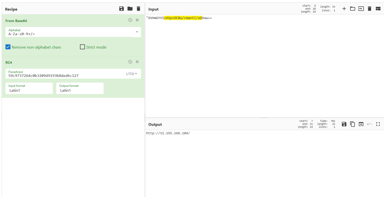
Figure 9: Raccoon v2 IP Address (via cyberchef utils)
