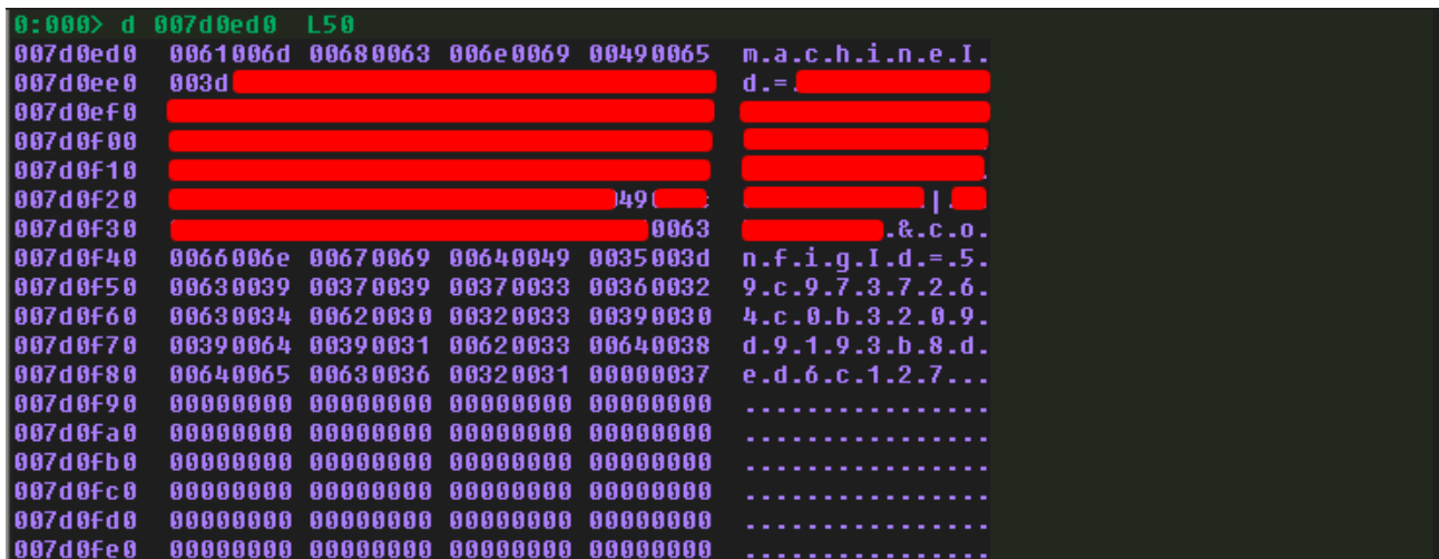
Figure 19: Raccoon v2: Fingerprinting Payload
