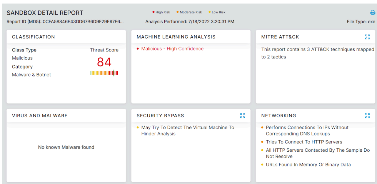
Figure 27: Zscaler Sandbox Detection
