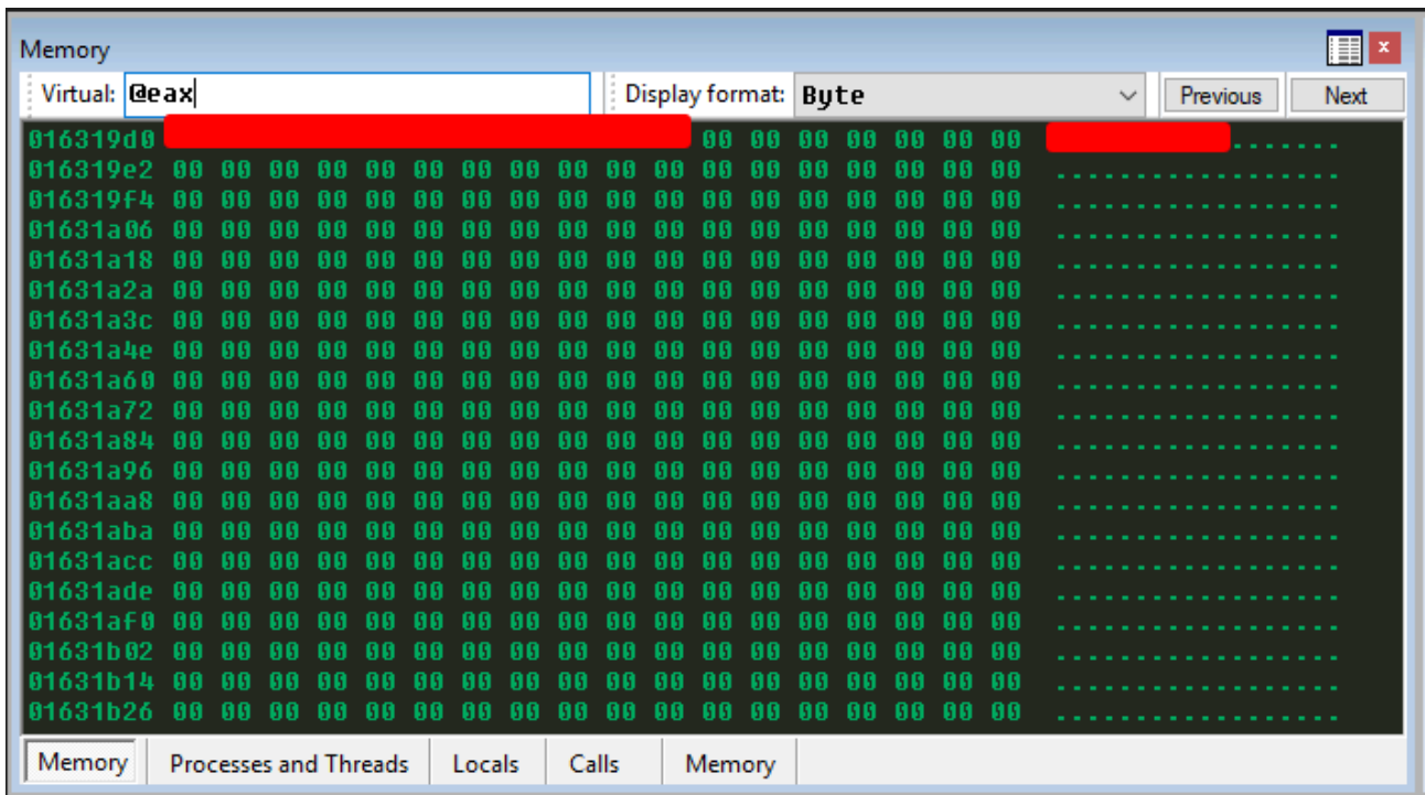
Figure 18: Raccoon v2: Username Buffer
