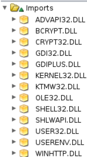
Figure 3: Raccoon Stealer v1 imports (unpacked)
